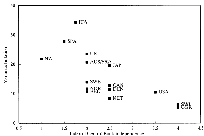
FIG. 1b. Variance Inflation
